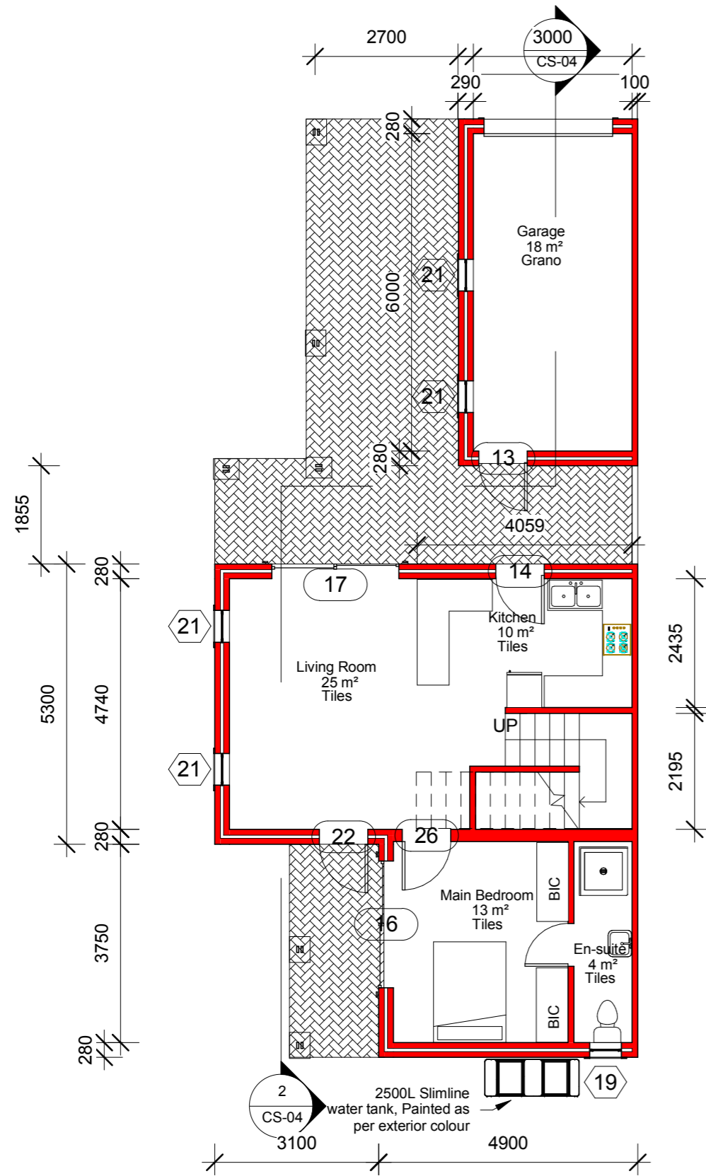
4 01 Ground Floor 1 : 100
