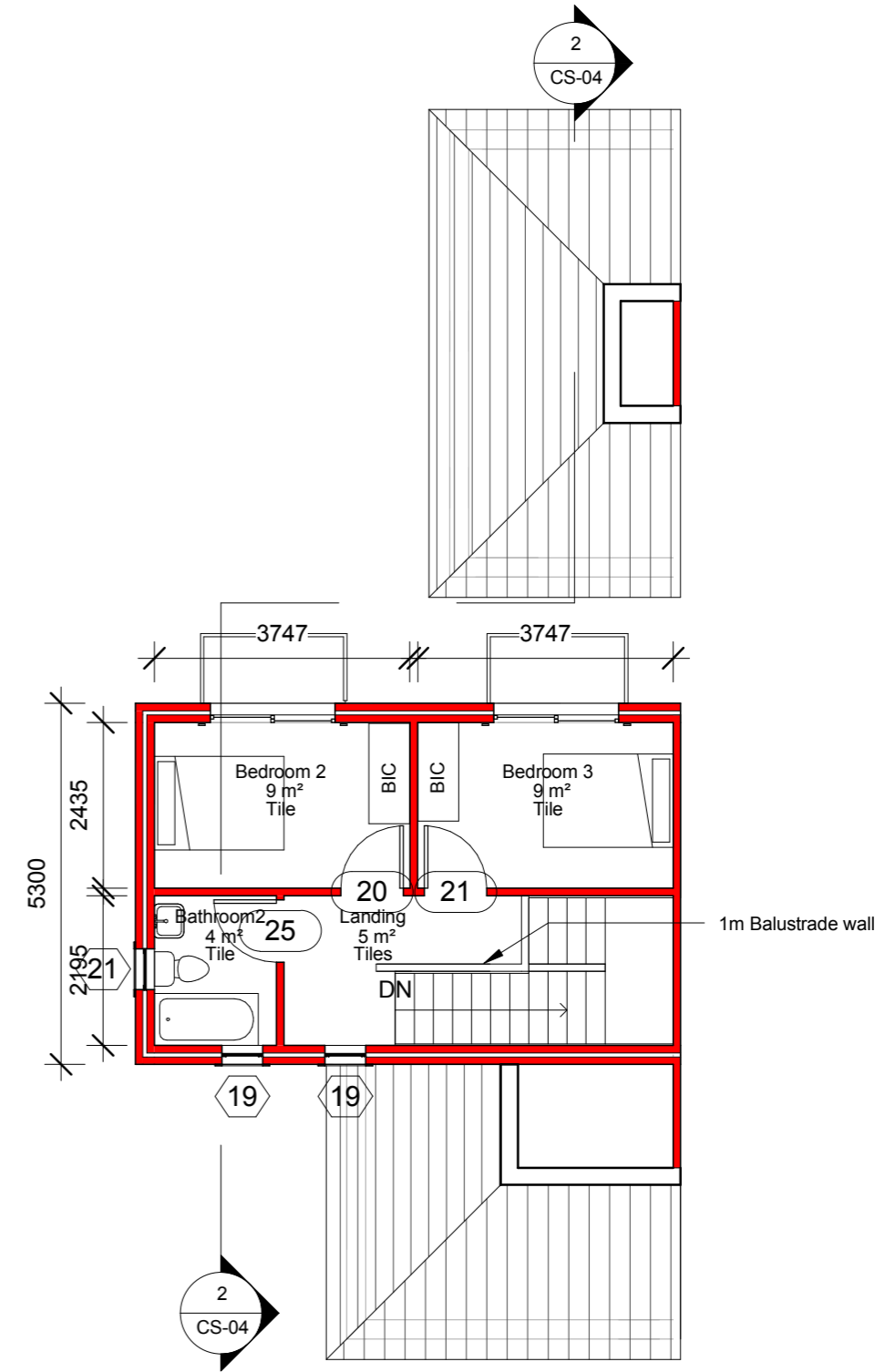
1 02 First Floor 1 : 100
